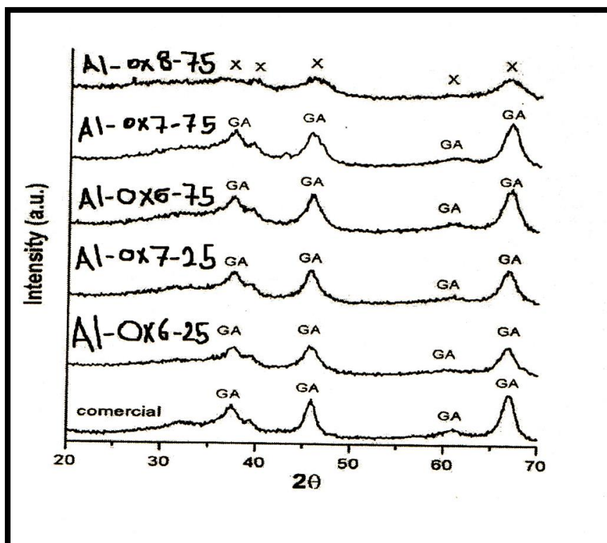
Fig. (4) : XRD patterns of different types of aluminas synthesized in this work and a commercial alumina ( GA: \gamma - Al_2O_3 ; \chi ; Chi- Al_2O_3 ).
