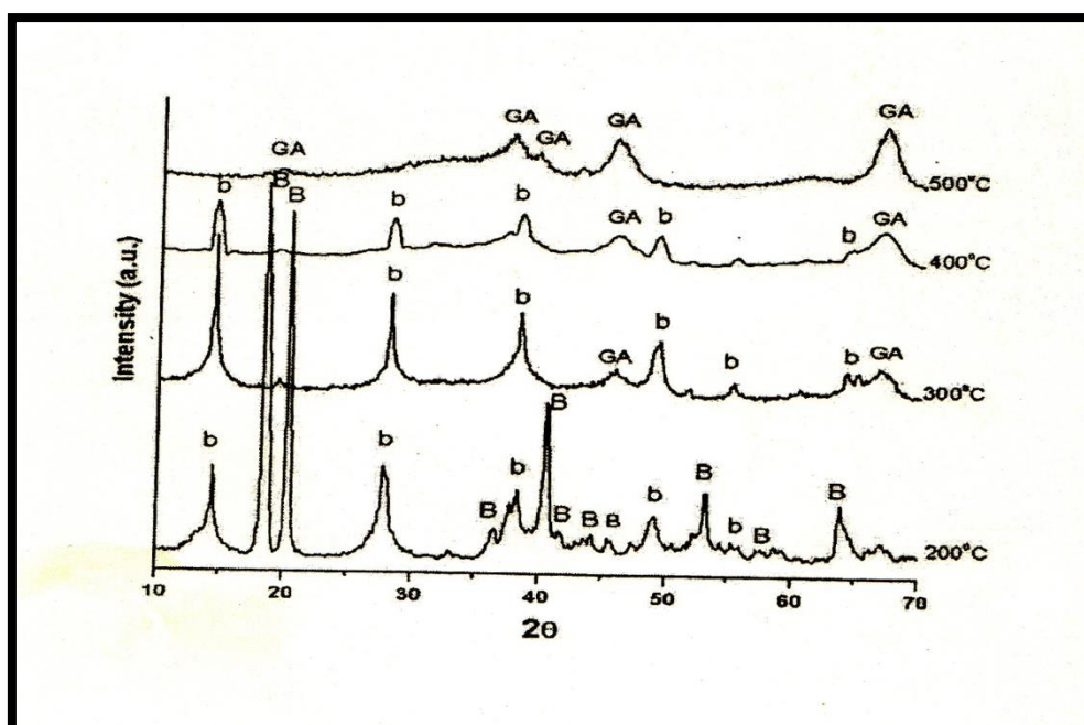
Fig.(3): XRD patterns showing phases of alumina formed during calcination of (G7-75) (B:bayerite; b;boehmite; G:gibbsite ; GA : \gamma - Al_2O_3 ) .
