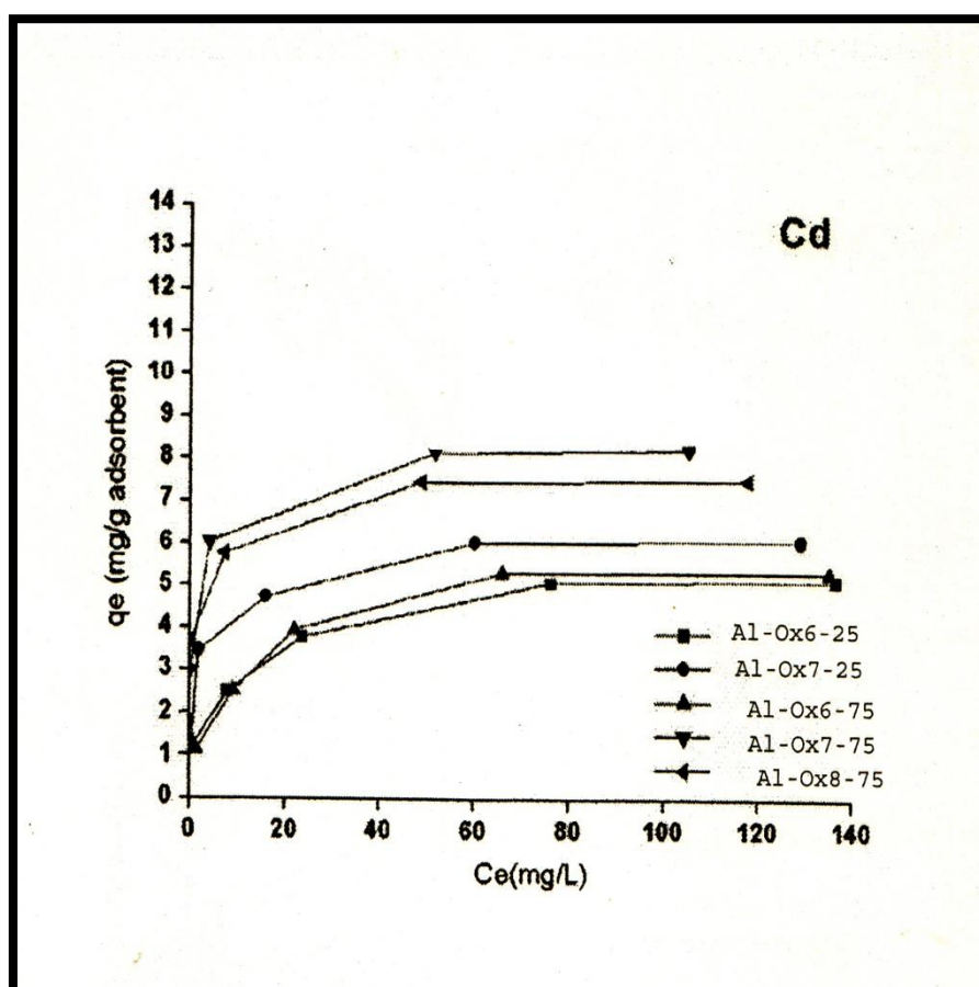
Fig.( 8a) : Adsorption isotherms obtained on activated alumina under various conditions .(a) cadmium .
