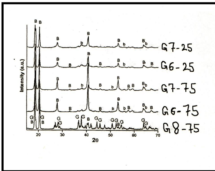
Fig.( 1 ) : XRD patterns of aluminum hydroxides synthesized under various conditions of aging temperature and pH of precipitation ( B:bayerite; b;boehmite; G:gibbsite ).
