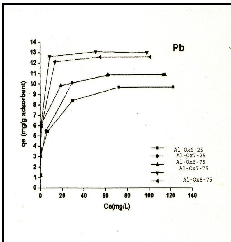
Fig. ( 8b) : Adsorption isotherms obtained on activated alumina under conditions .(b) Lead.
