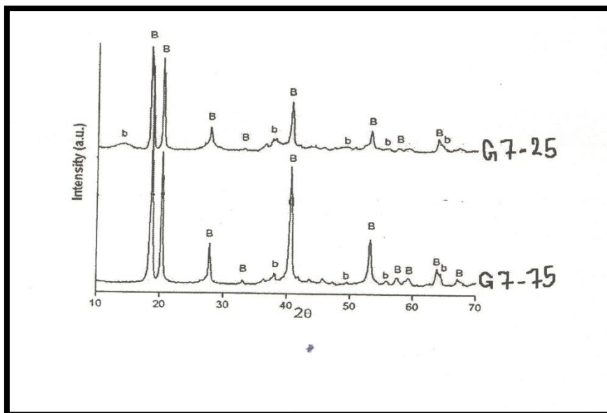
Fig.( 2 ) : XRD patterns of aluminum hydroxides aged under various conditions (B:bayerite; b;boehmite; G:gibbsite) .
